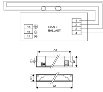
Specificaties Philips HF-S 158 TL-D II 220-240V
